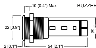
BUZZER UNITS
