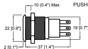
PUSH-BUTTON SWITCHES
